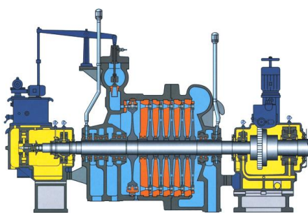
Back-pressure turbine
