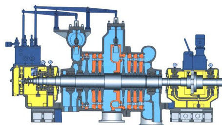
Extraction and condensing turbine
