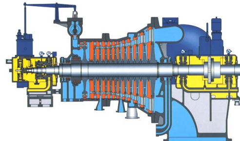
Condensing turbine
