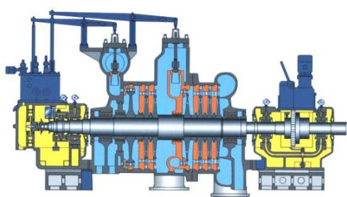
Extraction and back-pressure turbine
